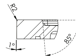
DETAIL F SCALE 1 : 3
