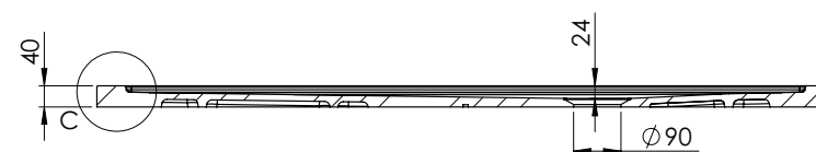
SECTION B-B
