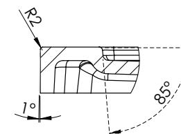
DETAIL C SCALE 1 : 3
